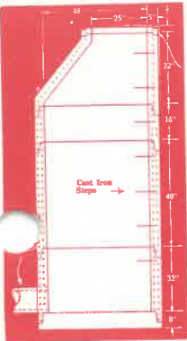
● PRE-CAST MANHOLES
