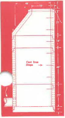
● PRE-CAST MANHOLES
